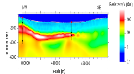
Figure 7: MT inversion (TE+TM)
