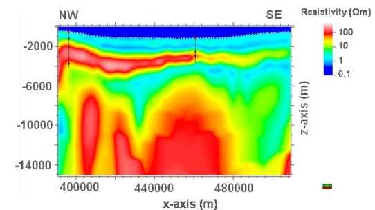
Figure 9: 2D CSEM+MT joint inversion from West of Shetland.
