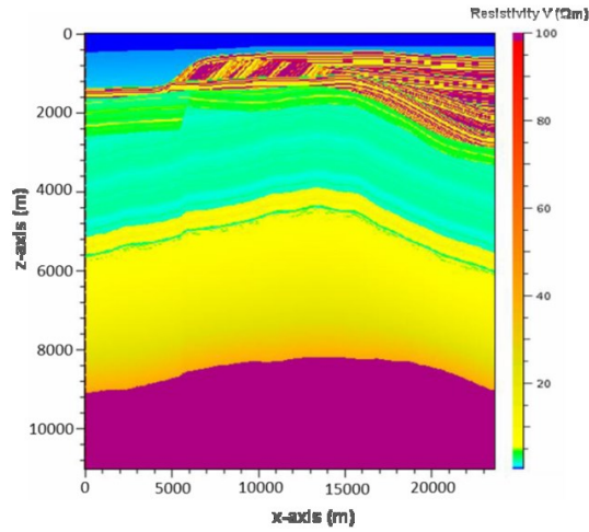
Figure 1: Vertical resistivity section of synthetic basalt model with detailed internal structure (after Herredsvella et al., 2012)
