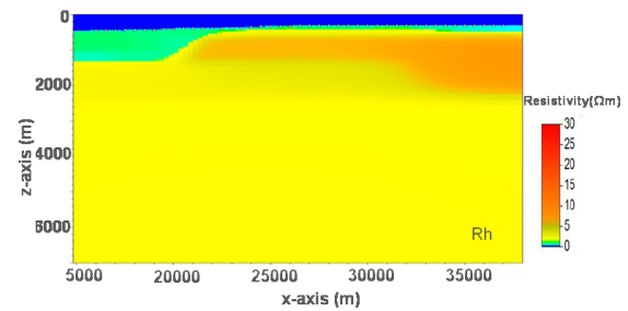
Figure 3: Horizontal resistivity model after 2.5D CSEM inversion.
