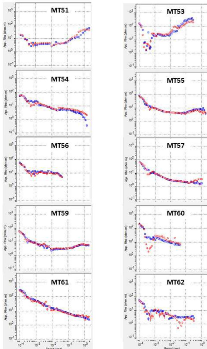
Fig.4. Resistivity curves of MT stations collected at different part of Thar desert, Rajasthan details of which are given in Table-1
