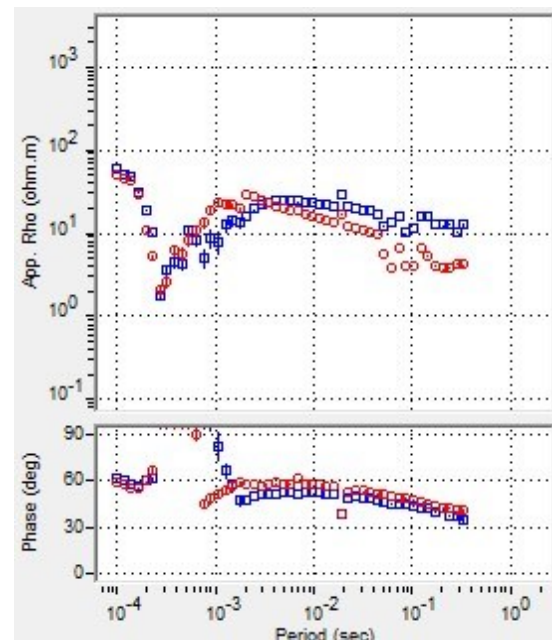
Fig. 2. Resistivity-phase curve of MT50.
