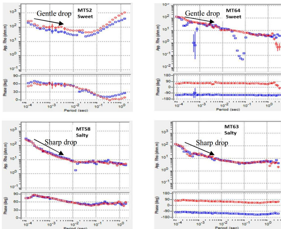
Fig.3. Resistivity Phase curves of MT52 (top left) data recorded at an offset of 200m from a sweet water tube well. MT64 (top right) data collected side by side of a sweet water tube well. MT58 (bottom left) data collected at an offset of 500m from a salty water tube well and MT63 (bottom right) data recorded at an offset of 100m from a salty water tube well.
