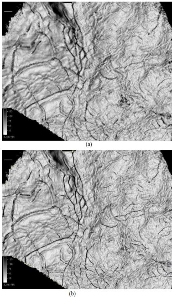
Figure 8 Polar dip attribute on (a) DSMF and (b) FES data. Polar dip using FES data brought out network of faults and fractures at greater extent.
