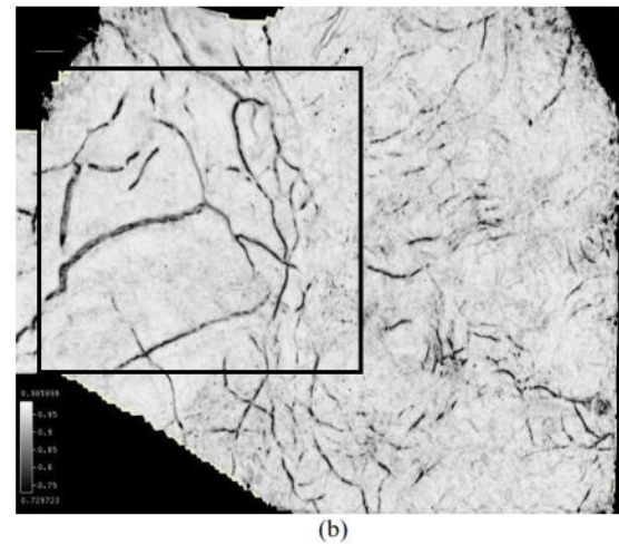
Figure 4 Minimum Similarity maps using (a) DSMF (b) FES data. Note that the area highlighted with square in both the maps, Minimum similarity using Fault enhances filter shows better definitions of faults and fractures.
