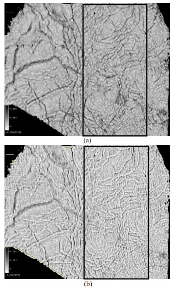
Figure 9 Most Positive Curvature using (a) DSMF and (b) FES data.
