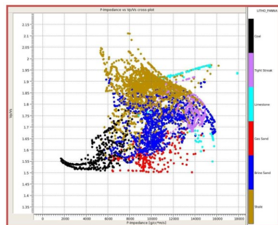
Fig. 5: P-impedance vs V_p/V_s cross-plot. No clear discrimination of gas bearing sands are possible.
