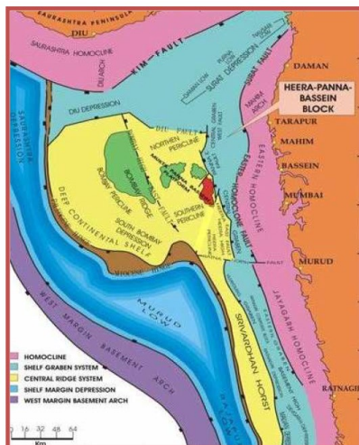
Fig. 3: Tectonic map of Heera-Panna-Bassein block
