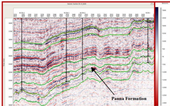
Fig. 6: Seismic section (Angle stack: 50-120) through arbitrary line passing through wells
