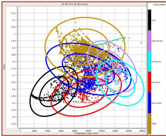
Fig.10: 2D normal probability distribution functions (pdfs) fitted to all identified litho-types within Panna formation in P-impedance vs Vp/Vs cross-plot
