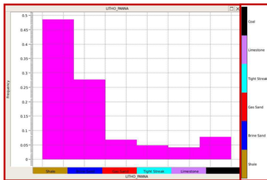
Fig. 11: Histogram of litho-facies proportions within Panna formation derived from wells in the study area
