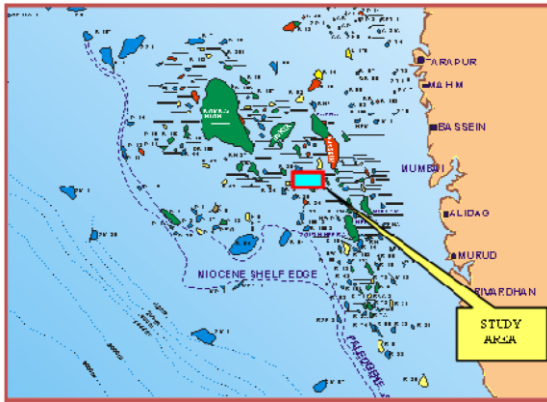
Fig. 2: Location of the study area within Heera-Panna-Bassein block of Western Offshore Basin
