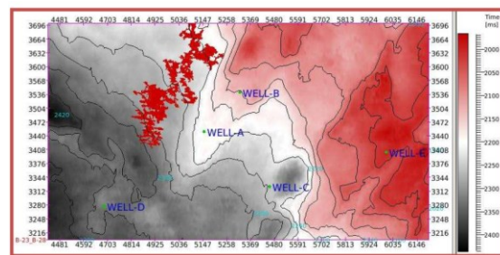
Fig. 13: Map view of probable gas charged geo-body superimposed on Panna top horizon
