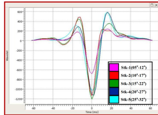
Fig. 8: Estimated composite wavelets for all five stacks.
