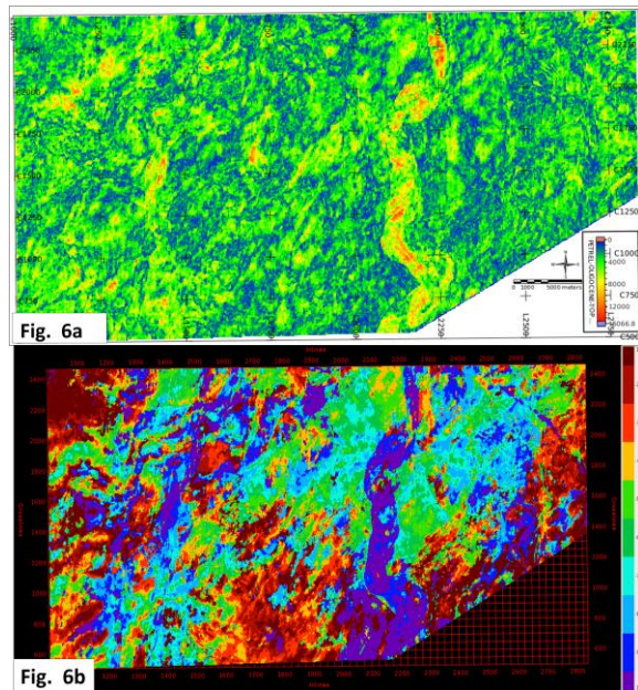
Figure 6: Slices along horizon 'Within Oligocene 2'. a) RMS amplitude +/-4ms. b) Seismic facies around horizon
