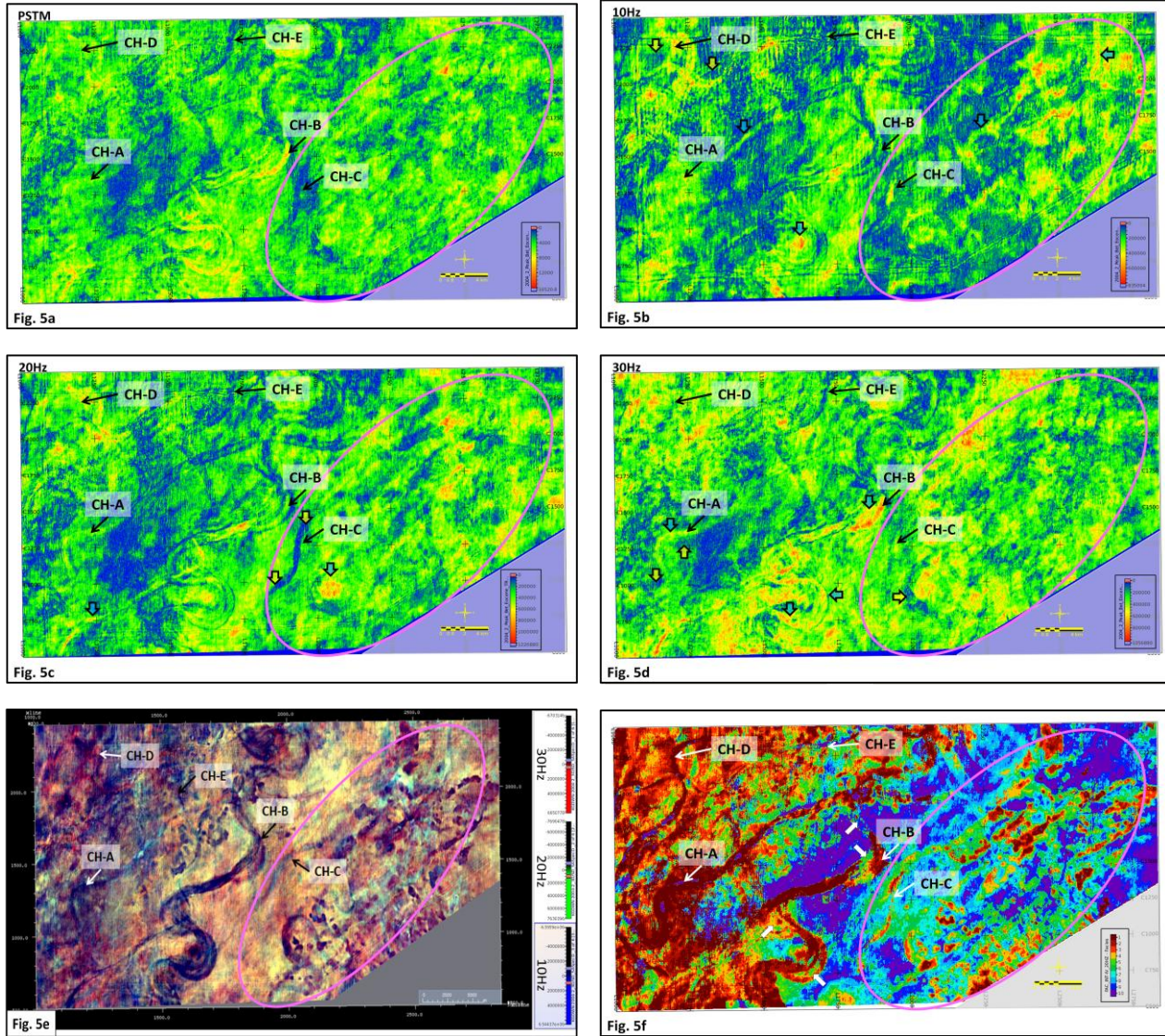
Figure 5: Slices along horizon 'Within Oligocene 1'
