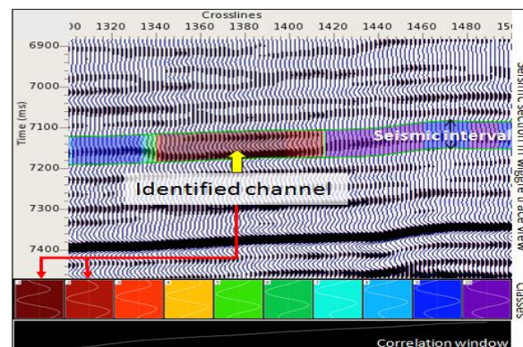
Figure 4: The seismic section showing 10 classes and similarity of seismic trace.
