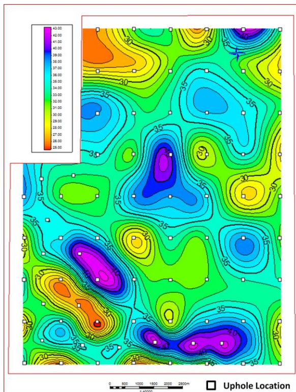
Figure-4: Finalized OD Map based on Uphole data before start of the production.
