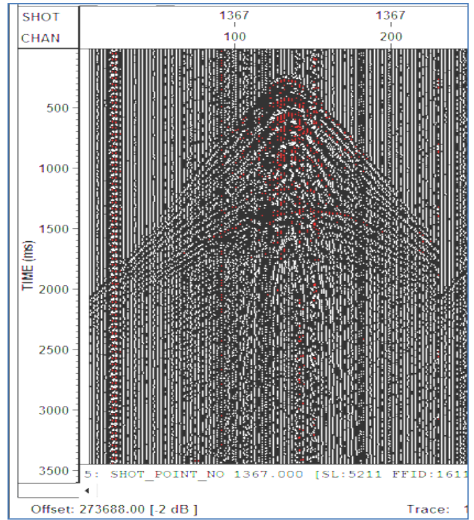
Figure-6 c: Test shot with depth – 42m & Charge Size- 5 Kg (Near Offset)
