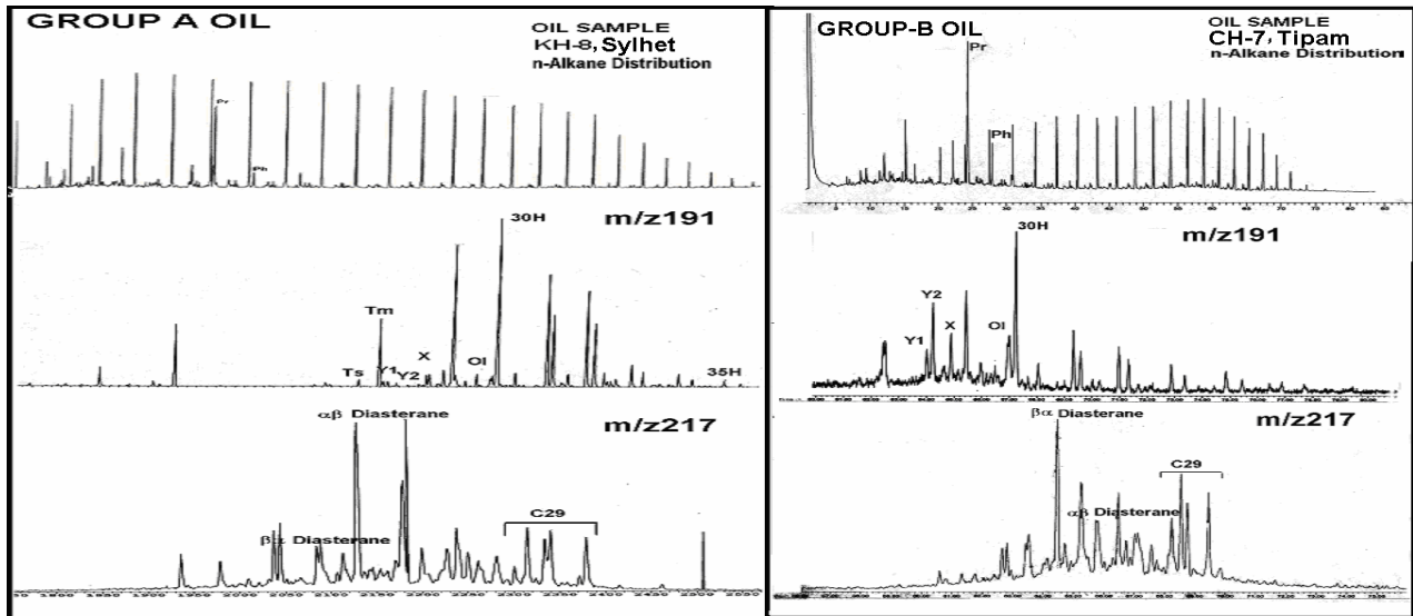
Fig. 9: n- alkane distribution, sterane and triterpane fingerprints for two oil groups
