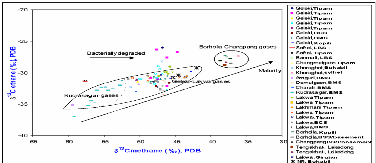
Fig. 10: Cross plot of \delta^{13}\text{C}_{\text{methane}} (‰), PDB vs \delta^{13}\text{C}_{\text{ethane}} (‰), PDB showing gas grouping of Assam
