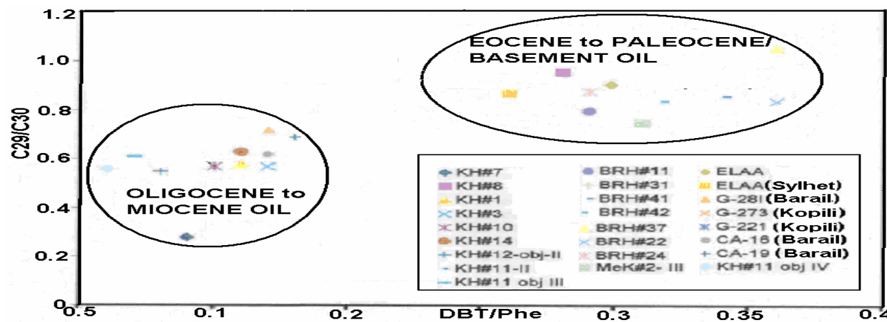
Fig. 8: Cross plot of DBT/Phe vs C29/C30 showing two oil groups
