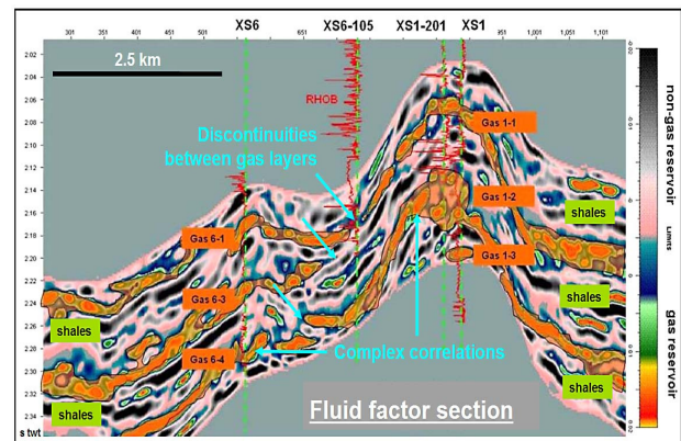
Figure 6: Fluid factor section from the PP-PS dual inversion. The three gas layers at identified at XS-1 & 6 are also evidenced by the positives value of the fluid factor. Thanks to 3C seismic the complex relationships between the two wells are established.
