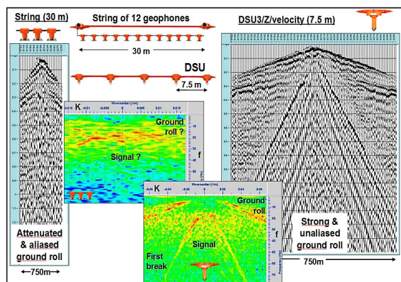
Figure 1: Shot points over the same offset range from arrays of geophones (left) and digital sensors (right). FK diagram shows that the prominent ground roll from single sensor data will be easily removed contrary to the aliased geophone data.
