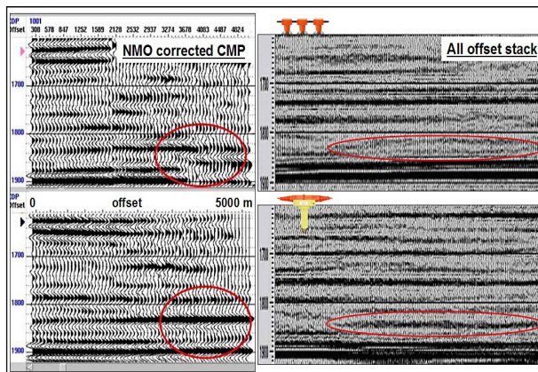
Figure 4: Comparison of NMO corrected CMP gathers and of the corresponding stacks between geophone arrays (top) and digital sensors (bottom). AVO at far offsets and corresponding amplitude anomaly on the stack are only preserved by single sensors.
