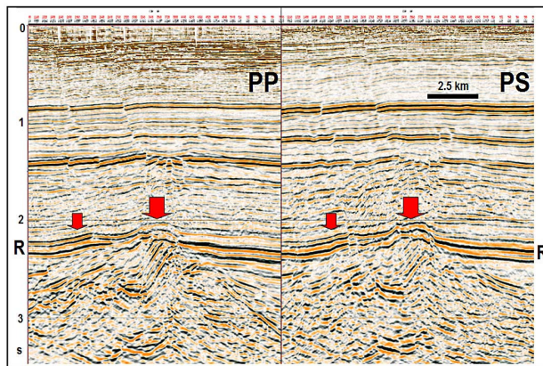
Figure 5: The PS migrated sections scaled to PP time is of sufficient quality to be compared with the PP one. Differences of amplitude at the top reservoir are evidenced on the two highs.
