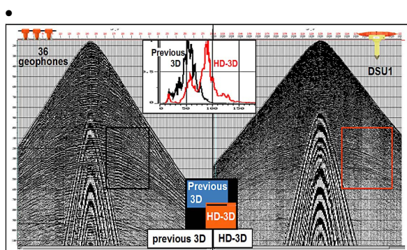
Figure 2: Comparison of SP's between array of geophones (left) and digital sensors (right), and the corresponding amplitude spectra. The main difference in HF content comes from the comparison of velocity with acceleration data. GR is attenuated by the array.
