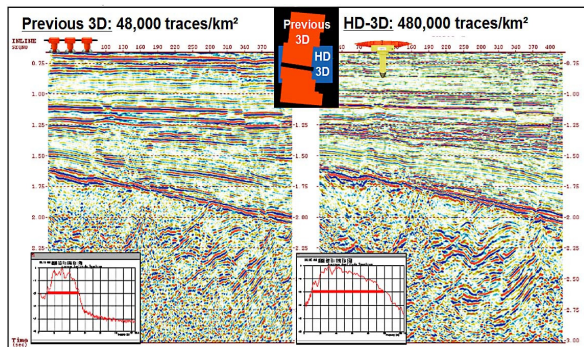
Figure 3: Comparison between two overlapping 3D surveys: one low density recorded by string of geophones (left section) and a new high density one recorded from digital sensors (right section). Both vertical resolution and signal-to-noise are improved (right).
