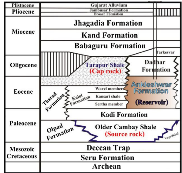
Figure 1: Schematic litho-stratigraphy distribution of the study area.
