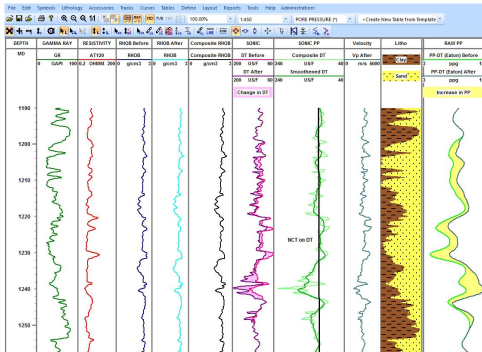
Figure 4: Representation of post CO 2 injection pore pressure envisaged using sonic logs recorded in the studied oil field, output taken from Pore pressure module, GEO suite of software.
