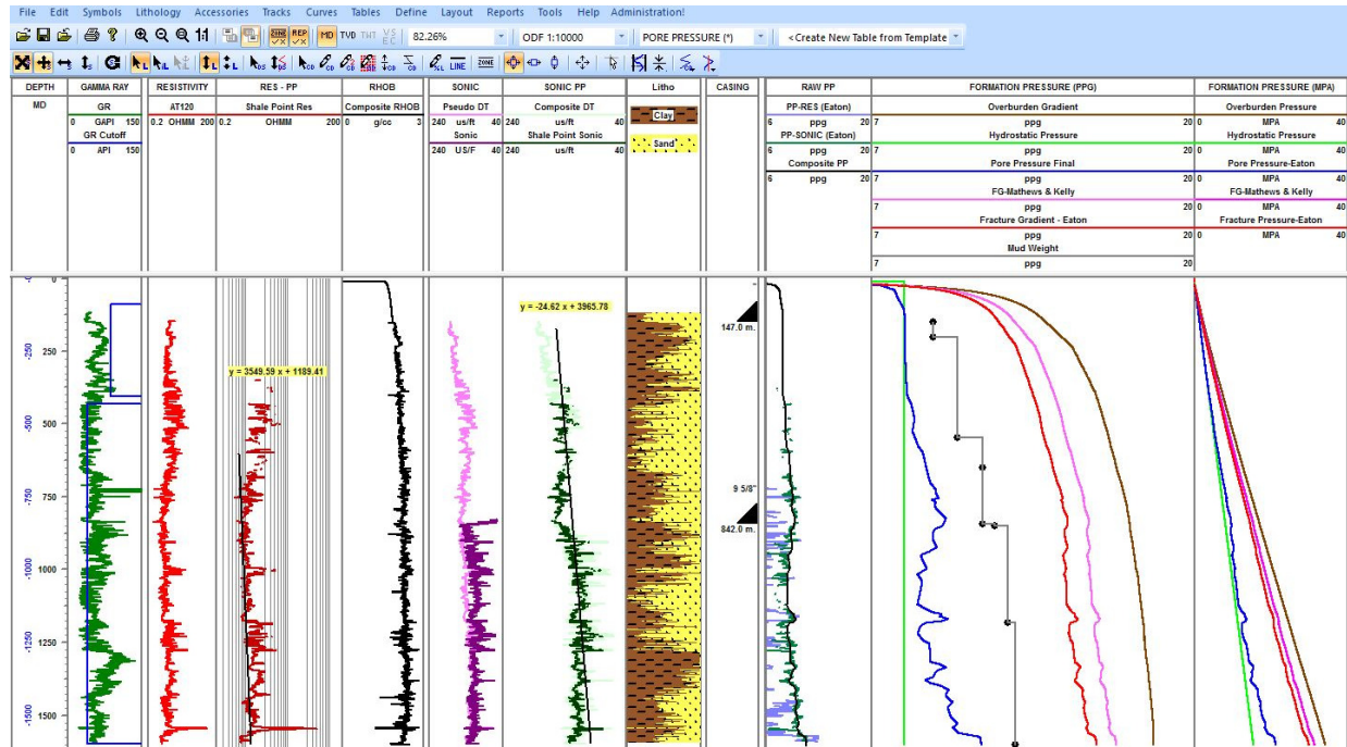
Figure 3: Estimated overburden, pore pressure, fracture pressure using resistivity and sonic logs recorded in the studied oil field, Ankleshwar in Cambay basin, output taken from Pore pressure module, GEO suite of software.
