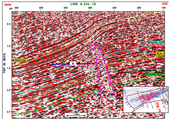
Figure 2: Seismic section displaying the potential zone for CO 2 injection, S_{3+4} , from the study area (ONGC India Pvt. Ltd, personal communication).
