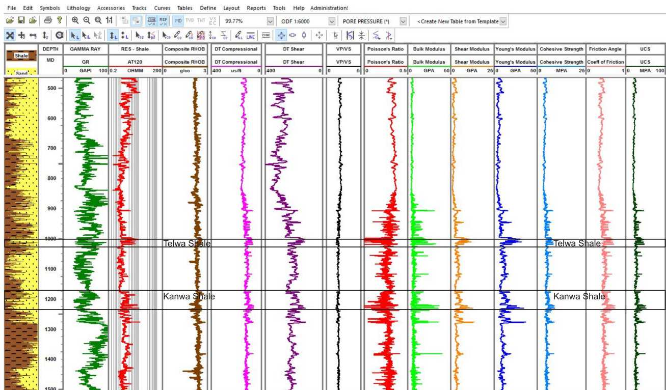
Figure 5: Computed shear sonic slowness, geomechanical moduli and UCS from one of the studied wells. The cap rocks, Telwa and Kanwa shales are marked by black colour boxes, output taken from pore pressure module, GEO suite of software.
