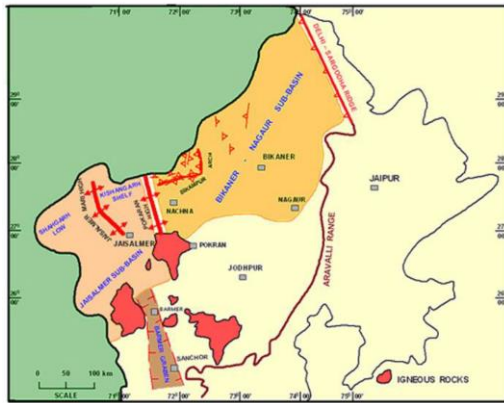
Fig.1: Geological map of Pariwar Formation.
