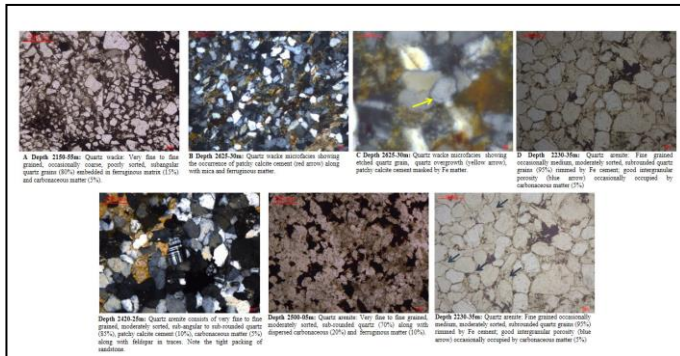
Fig.2: Petrographic attributes of Pariwar Formation
