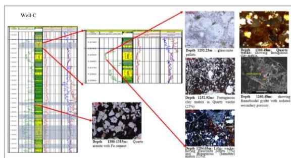
Fig.10: Petrographic attributes showing presence of glauconite, Fe cements, and chloritic matrix in sandstones of Pariwar Formation in well-C
