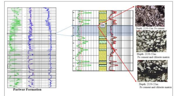
Fig.:7: Petrographic attributes showing Fe cements and chloritic matrix in sandstones of Pariwar Formation of well-A
