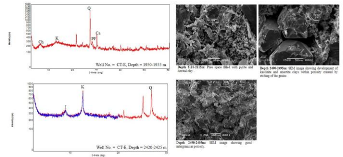
Fig.3: XRD and SEM attributes of Pariwar Formation
