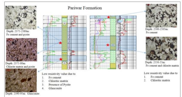
Fig.:8: Petrographic attributes showing glauconite, Fe cements and chloritic matrix in sandstones of Pariwar Formation of well-A
