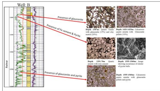
Fig.9: Petrographic attributes showing presence of glauconite, Fe cements, and chloritic matrix in sandstones of Pariwar Formation in well-B
