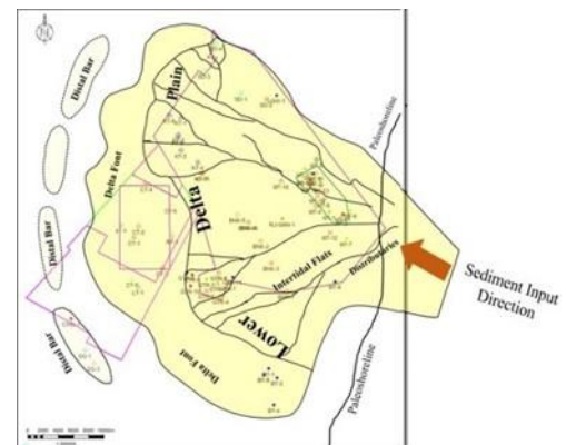
Fig.6: Facies map of Pariwar Formation
