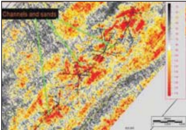
Fig. 5: Arc length extraction over the whole Zone II reservoir interval for the central part of the South Tapti Field, showing the presence of sands and channel geometries.
