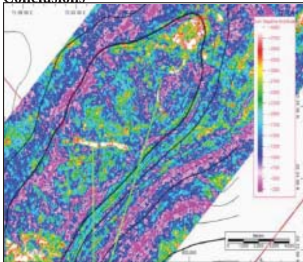
Fig. 10: Sum of negative amplitudes map over the whole Zone II-C reservoir interval for the central part of the South Tapti Field, indicating the distribution of the sands within Zone II. Pink to yellow colour scale represent the increasing negative amplitudes.
