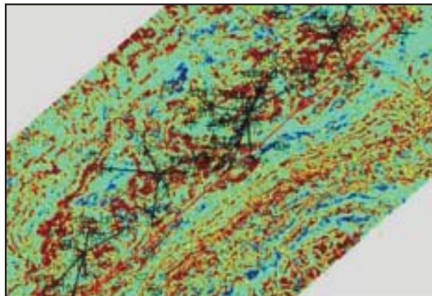
Fig. 8: Number of zero crossings attribute analysis over the whole Zone II reservoir interval for the central part of the South Tapti Field, indicating the extent of shale interbedding within Zone II.
