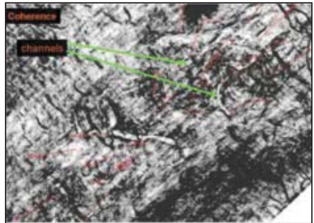
Fig. 6: Coherency extraction over the whole Zone II reservoir interval for the central part of the South Tapti Field, projected onto an horizon slice, showing detail of Zone II the channel geometries.
