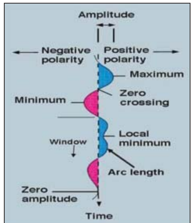
Fig. 4: Arc Length defined as the length of the seismic waveform over a given window.
