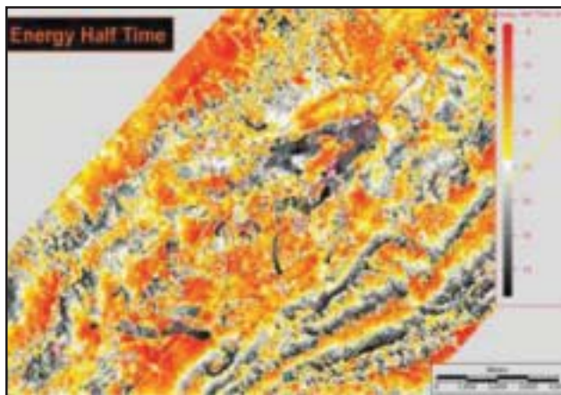
Fig. 7: Energy half-time analysis over the whole Zone II reservoir interval for the central part of the South Tapti Field, indicating the distribution of the sands within Zone II.
