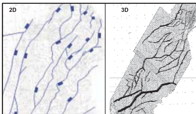
Fig.2 Map showing fault pattern based on 2D (on the left) & 3D (on the right)
