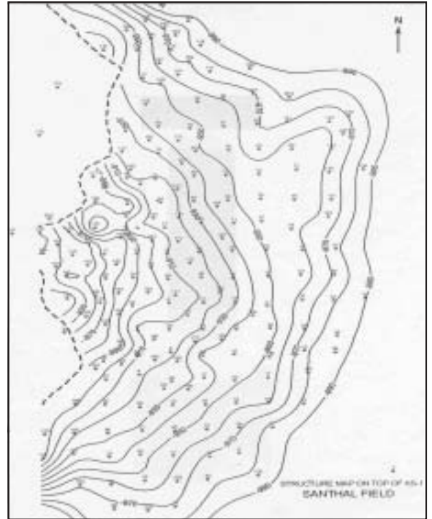
Fig-9 Structure Map on top of KS-1 (without Fault)
