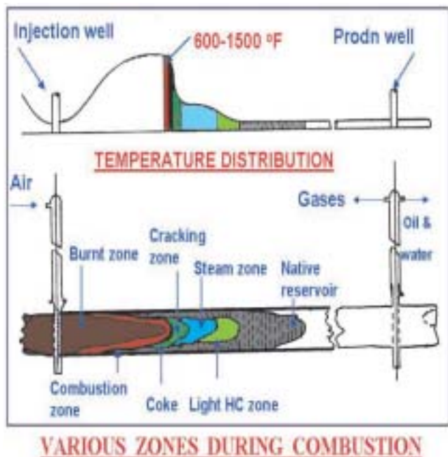
Fig-2 Schematic Diagram of In-Situ Combustion
