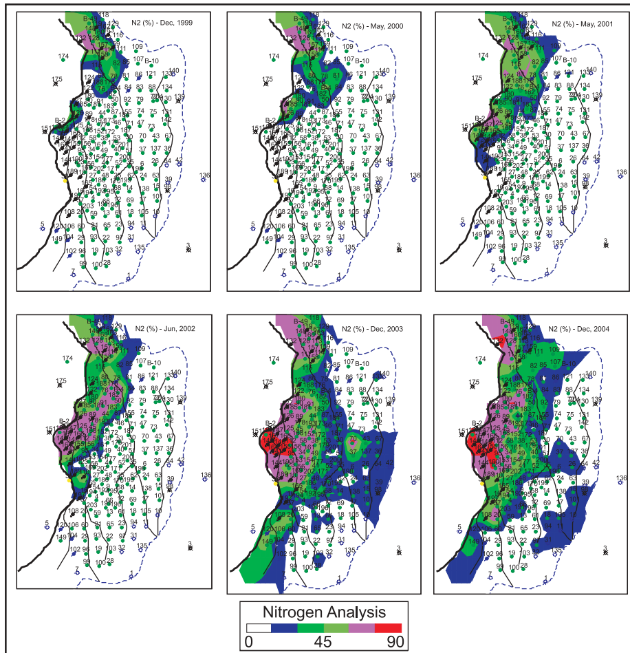
Fig 10: Time lapsed EOR influenced Area (Based on gas analysis from 1999 to 2004)
