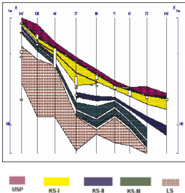
Fig-3 Cross Section W-E (Central Part)
