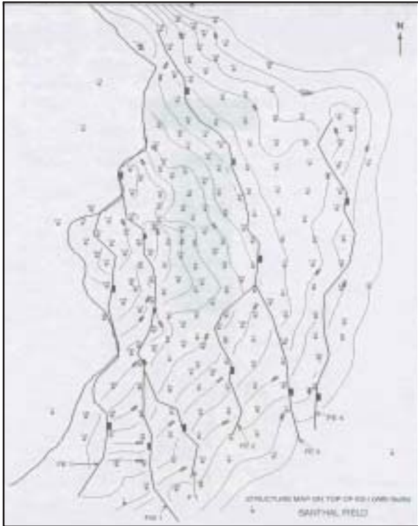
Fig. 8 : Structure map on top KS-1 with fault
