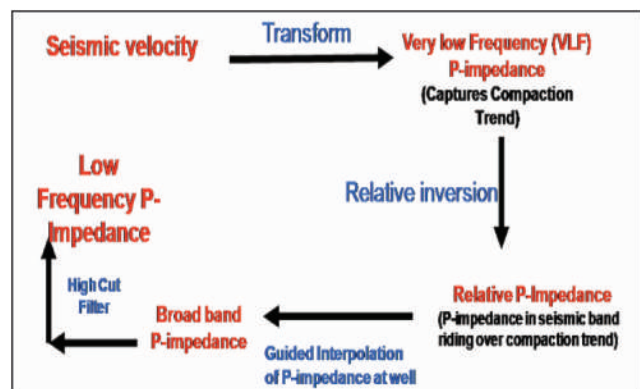
Fig. 6: Low Frequency Modeling workflow
