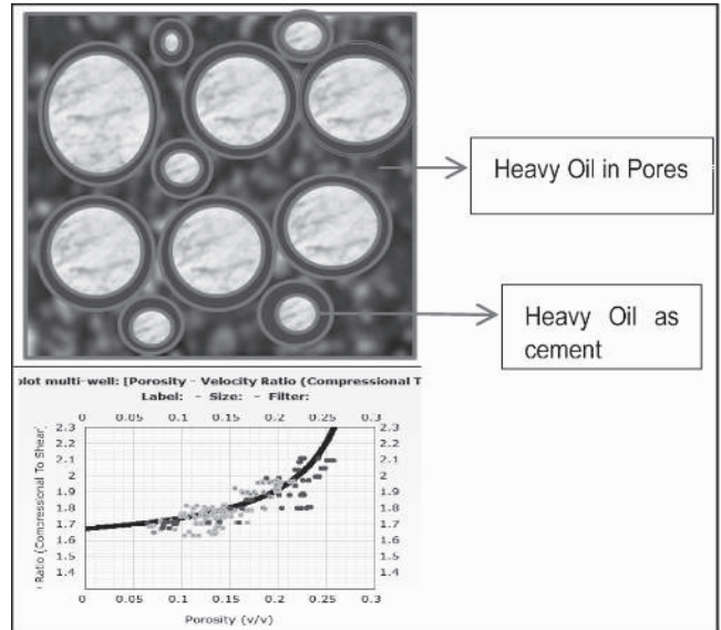
Fig. 3: The figure above explains the rock physics model and the match of the model with the observed well data
