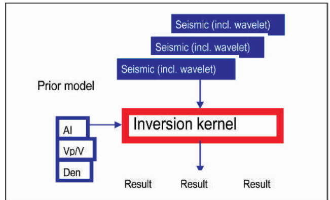
Fig. 4: Simultaneous AVO inversion workflow
